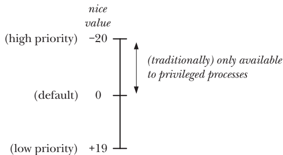
Figure 35-1: Range and interpretation of the process nice value
